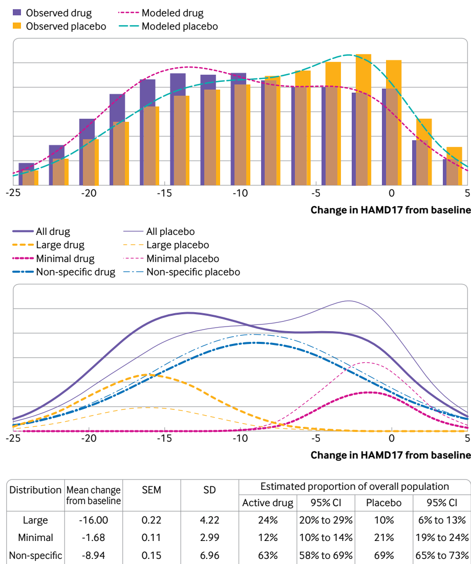
Fig 2 | (Top) Fit of the mixture model distributions (curves) for drug and placebo responses with the respective histograms for the observed drug and placebo responses. (Bottom) Overall finite mixture model and component normal distributions for drug and placebo. HAM-D17=Hamilton rating scale for depression; SEM=standard error of the mean; SD=standard deviation
