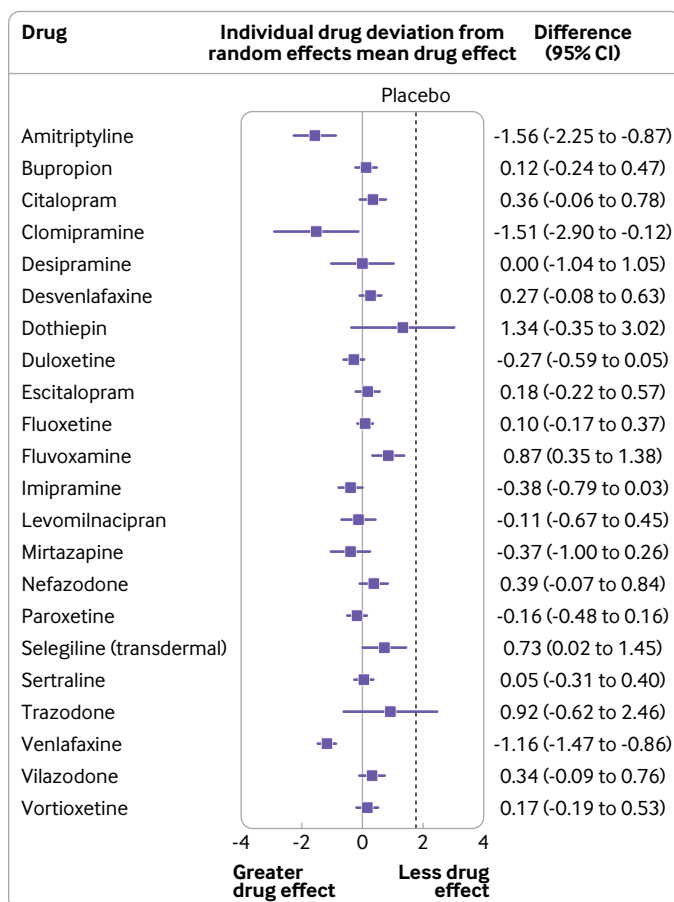
Fig 3 | Estimated effect for each drug. Center line shows the overall (random effects) mean effect for active drug to show how each drug differs from the average. Placebo line is a reference for how the differences among drugs compare with the differences between drugs and placebo
