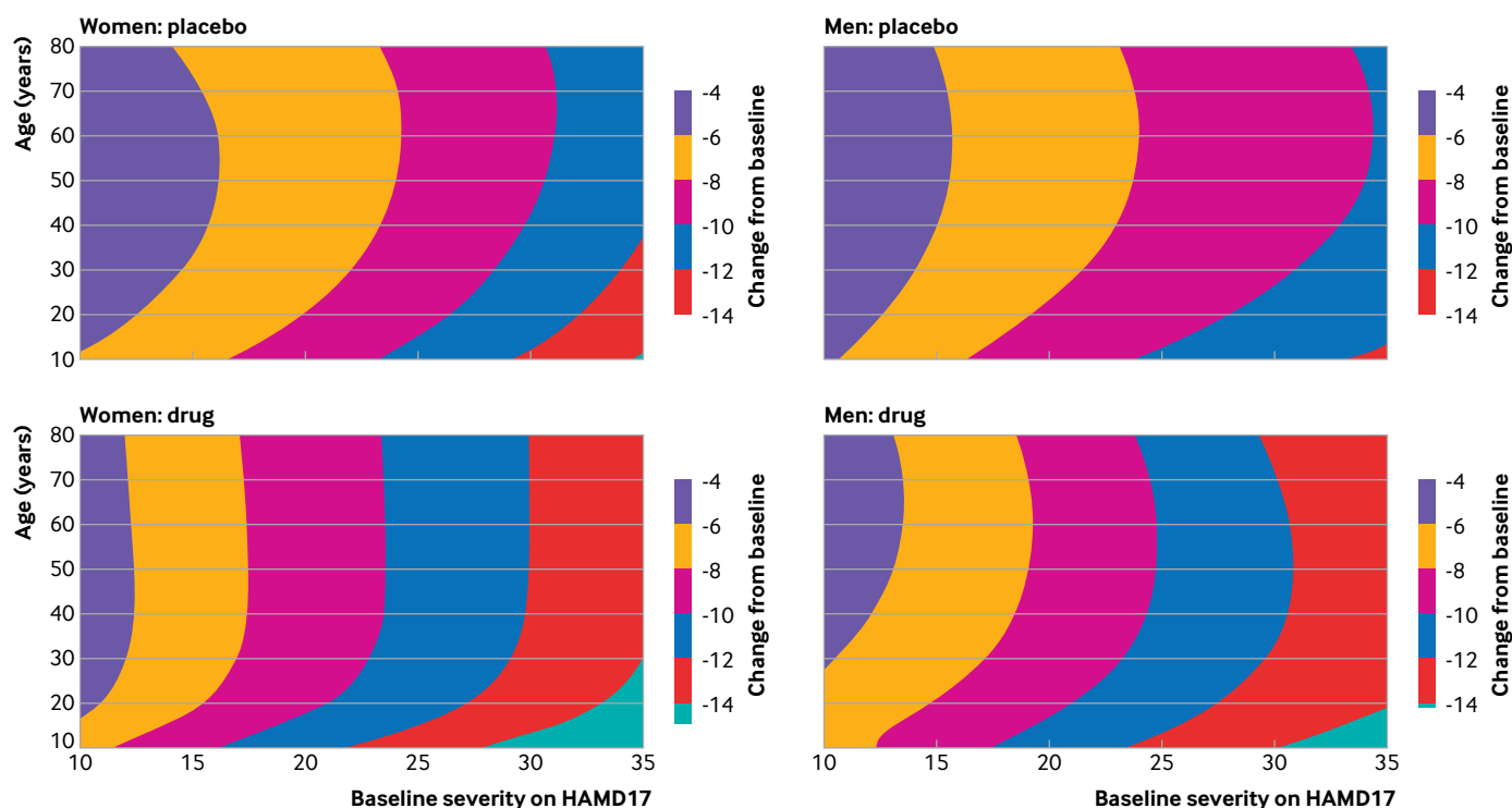
Fig 1 | Heatmaps showing predicted treatment responses (change from baseline) as a function of sex, age, and baseline severity on the Hamilton rating scale for depression (HAMD17)
